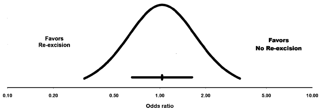
Fig. 4 Distribution curve of the true effect size, assuming a normal distribution of effects (on a log scale). The plot illustrates the pooled odds ratio (OR), its 95% confidence interval (CI), and the prediction interval, which ranges from 0.319 to 3.354. This interval represents the range in which the true effect size is expected to fall in 95% of comparable populations. The central point reflects the pooled OR, while the thick horizontal line indicates the 95% CI. The extended horizontal line represents the prediction interval, accounting for between-study heterogeneity
