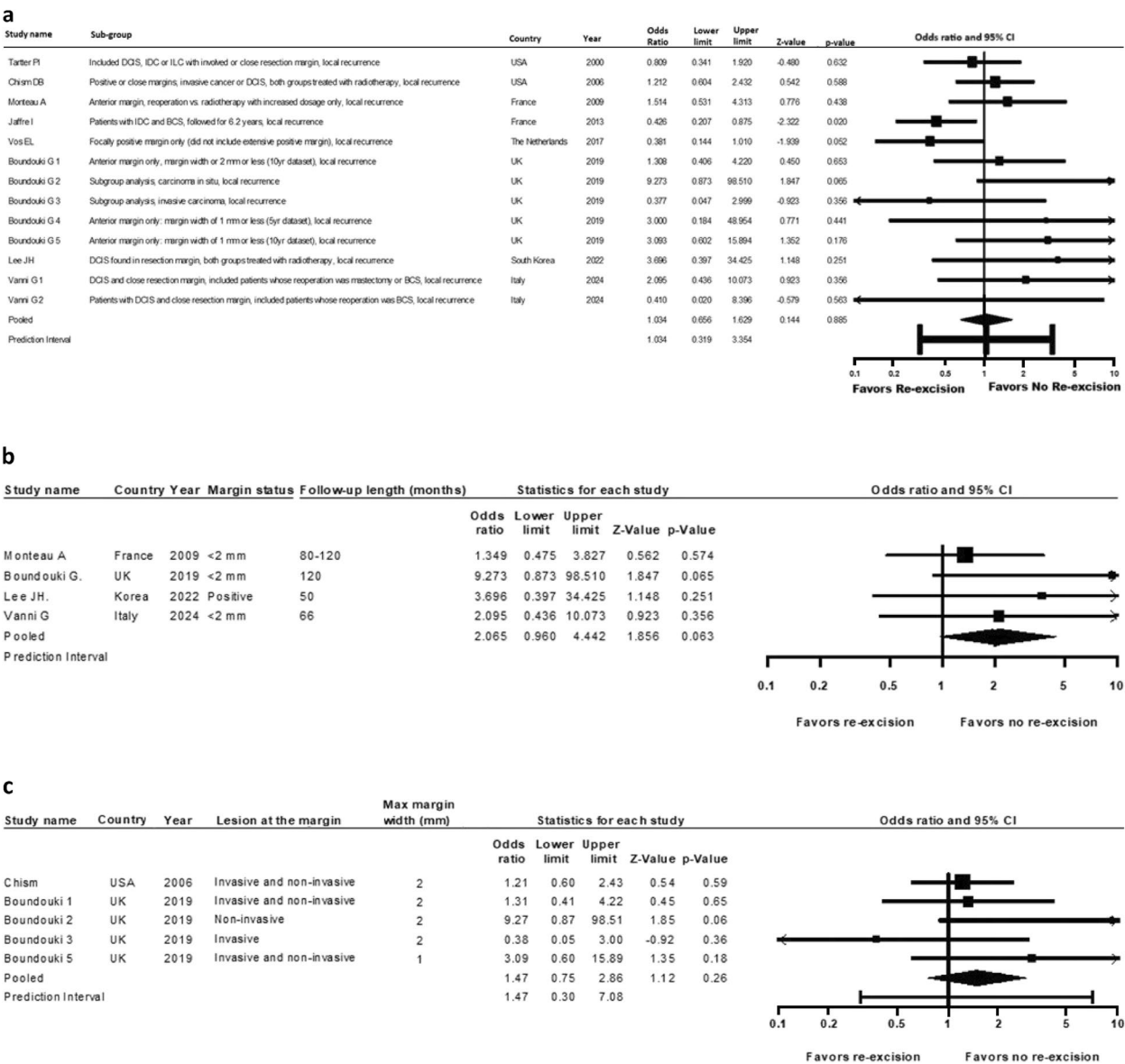
Fig. 2 a Forest plot of all datasets included in the meta-analysis, showing odds ratios (OR) and 95% confidence intervals (CI) for local recurrence after re-excision versus no re-excision. Each horizontal line represents the 95% CI for the individual study, and the box indicates the weight of each study in the meta-analysis. The diamond represents the pooled odds ratio and its 95% CI. A random-effects model was applied to account for potential heterogeneity between studies. DCIS = ductal carcinoma in situ; IDC = invasive ductal carcinoma; ILC = invasive lobular carcinoma; BCS = breast-conserving surgery. b Forest plot of the subgroup meta-analysis for studies and datasets that included only patients with ductal carcinoma in situ (DCIS). Each horizontal line represents the 95% confidence interval (CI) for an individual study, and the box indicates the weight of the study in the meta-analysis. The diamond represents the pooled odds ratio (OR) and its 95% CI. A random-effects model was applied to account for potential heterogeneity between studies. c Forest plot of the subgroup meta-analysis for studies and datasets including patients with ductal carcinoma in situ (DCIS) and invasive breast cancer (IBC), with approximately 10 years of follow-up. Each horizontal line represents the 95% confidence interval (CI) for an individual study, and the box size reflects the weight of the study in the meta-analysis. The diamond represents the pooled odds ratio (OR) and its 95% CI. A random-effects model was applied to account for potential heterogeneity between studies
