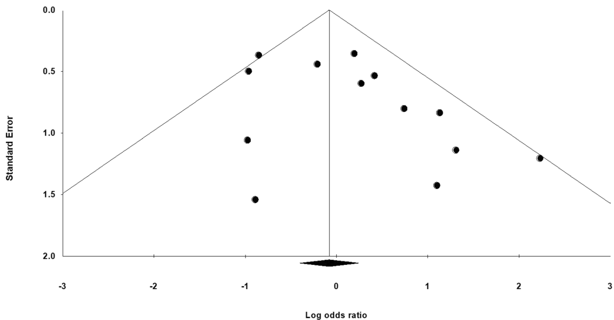
Fig. 3 Funnel plot assessing publication bias for the studies included in the meta-analysis. The vertical line represents the pooled effect size (log odds ratio), and the diagonal lines indicate the pseudo 95% confidence limits. Each dot represents an individual study. The symmetrical distribution of studies within the funnel suggests a low likelihood of significant publication bias
